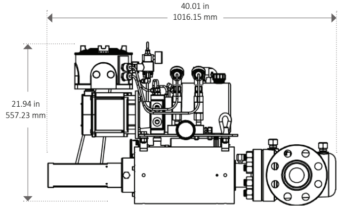
Valve shown installed in horizontal orientation. Operating stem and flow bore are horizontal. Vertical orientation is also available.
